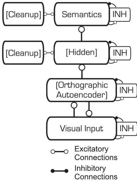
Figure 3: The architecture of the network used in Simulation 1. Names of hidden layers are in square brackets. The bottom two layers form a feedforward autoencoder with separate input and output layers, but these are depicted as a single “Visual Input” layer with bidirectional connectivity for simplicity.
