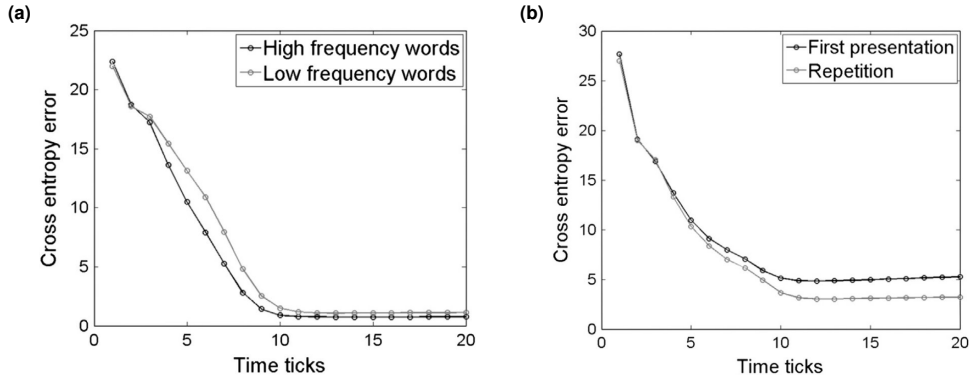
Figure 2: Rabovsky and McRae’s (2014) results using cross-entropy error to simulate the effects on N400 amplitude of (a) word frequency and (b) repetition. (Reprinted with permission from Rabovsky & McRae, 2014).
